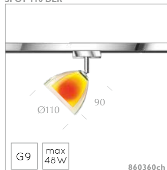
SILVA SPOT 110 DLR
