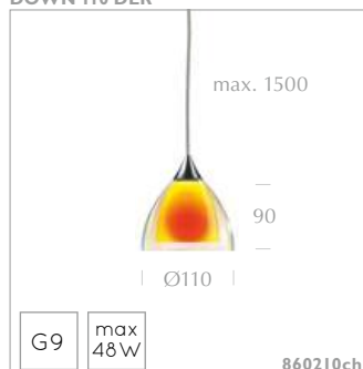
SILVA DOWN 110 DLR
