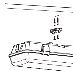
Surface installation
